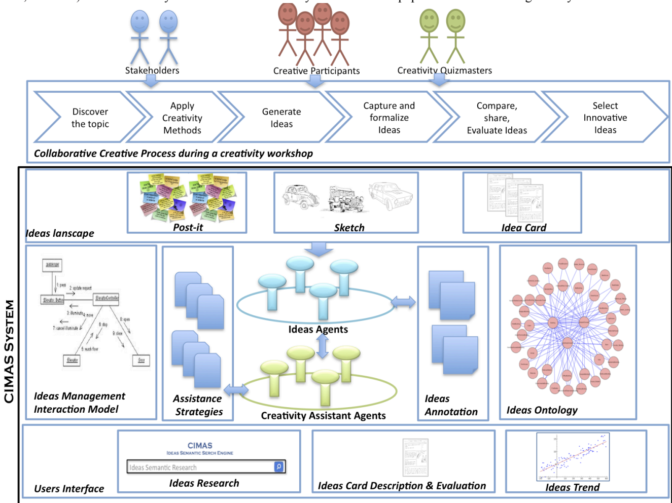
Fig. 2. CIMAS architecture
