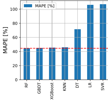
Fig. 7: Regression results for baseline feature set across different ML models.
