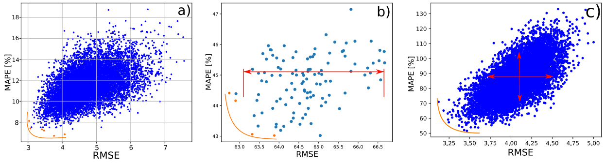
Fig. 6: RMSE vs MAPE results for a) CCS data set, b) CTADS - incident duration c) Random vectors
