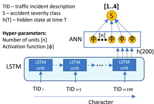
Fig. 3: LSTM sentiment encoder structure.
