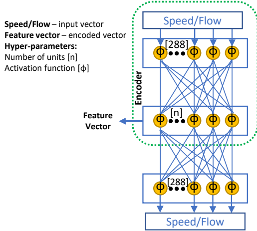
Fig. 5: The structure of the ANN autoencoder
