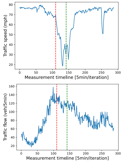
Fig. 1: a) Traffic speed and b) Traffic flow plots for the VDS associated to incident A-4798 (accident on US-101 Southbound with duration of 31 5-minute iterations - actual reported incident clearance time, without considering the incident recovery time). The red line denotes the start of the accident, and the green line the end of the accident. The blue line denotes the speed evolution in the vicinity of the incident location (drops almost to 20km/h) while the flow is still running at high values due to large numbers of vehicles blocked in traffic.
